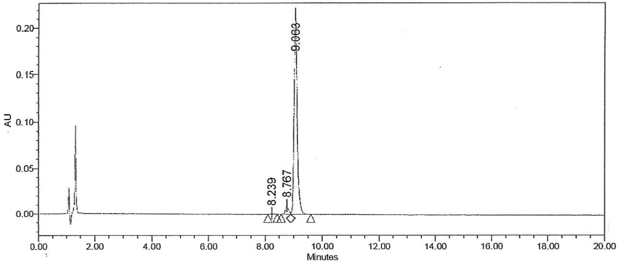
Auto-Scaled Chromatogram
